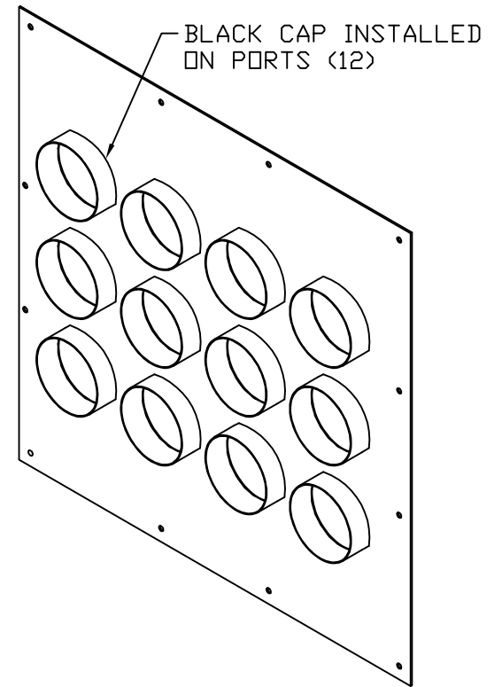
12 UNIT ENTRANCE PANEL 3X4 MAPLE POWDERCOAT FINISH
