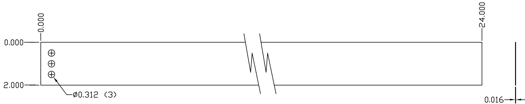
COPPER FLAT STRAP (1)
